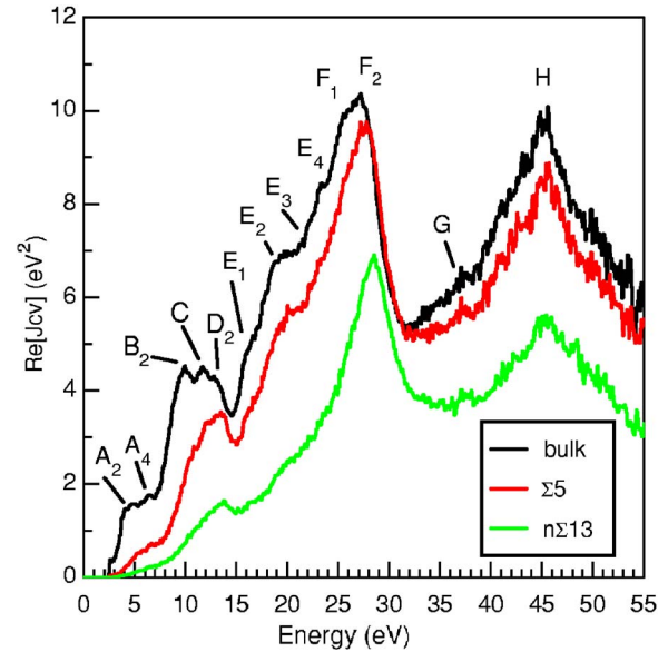
FIG. 2. (Color online) Interband transition strength spectra recorded from bulk \text{SrTiO}_3 as well as from the \Sigma 5 and the n\Sigma 13 grain boundary cores. Labeled transitions are assigned in Table I.
